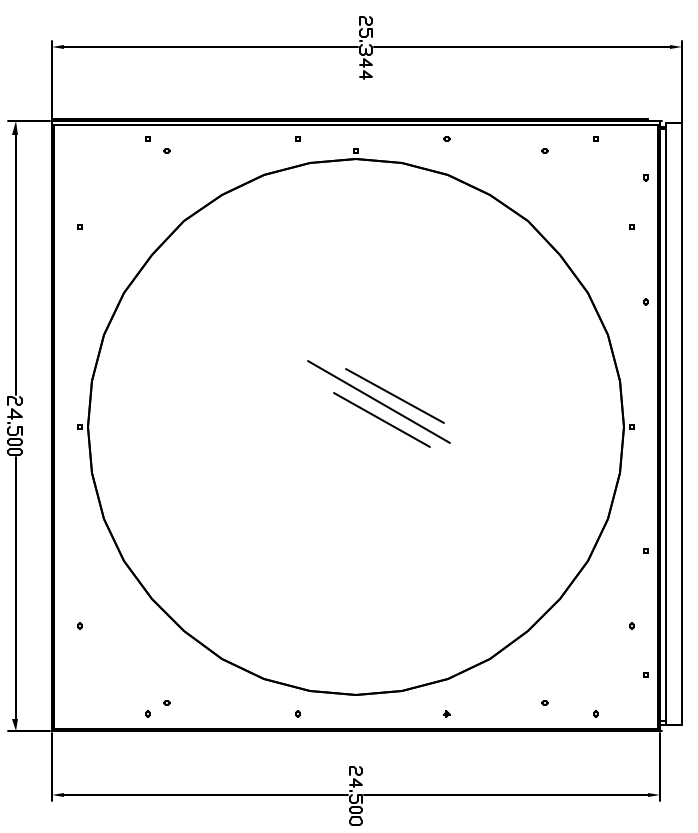
FRONT VIEW WITH DDDR AND TOP COVER
