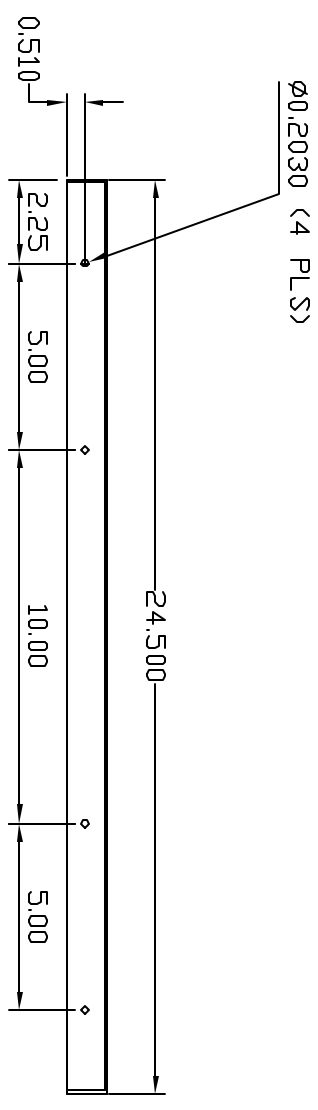
FRONT VIEW
